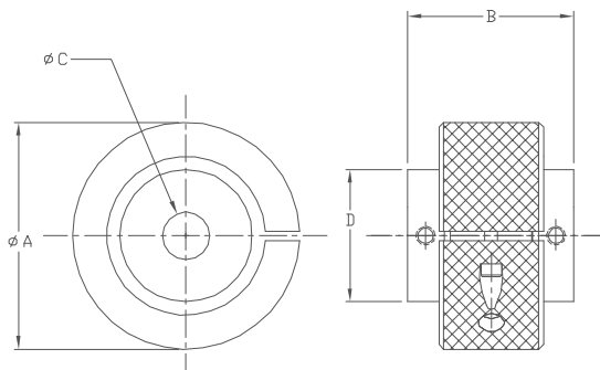
IN-LINE SHAFT
