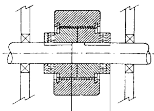
IN-LINE SHAFT
