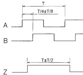
Output Waveform
