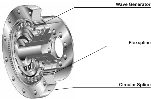
Structure of Harmonic Drive® component product
