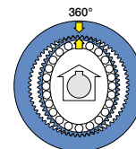
One Turn of Wave Generator
