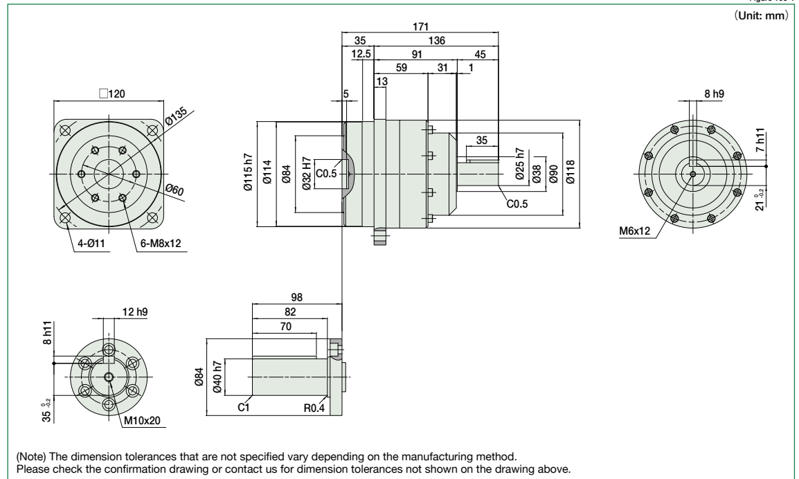
HPG-50 Outline Dimensions
