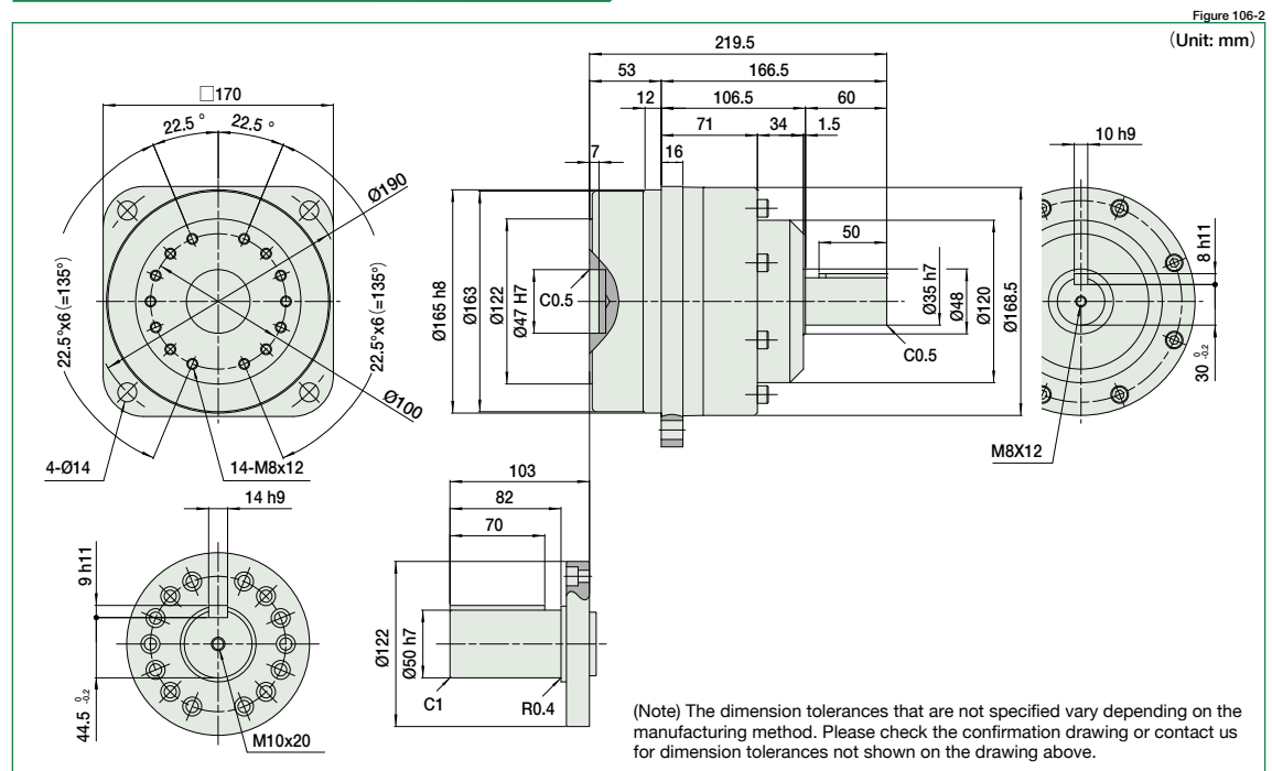
HPG-50 Outline Dimensions
